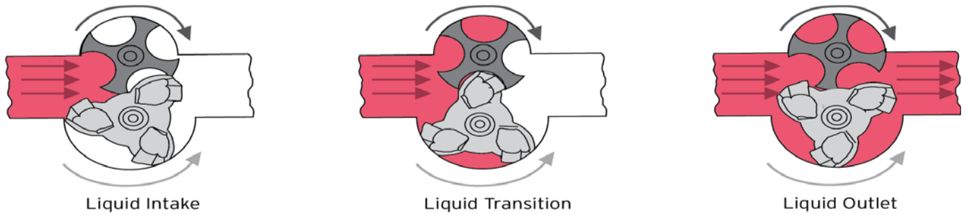
Figure 1 - BiRotor Meter Principle of Operation Diagram
